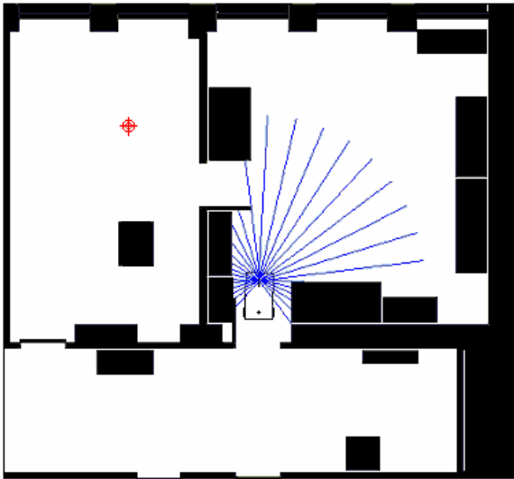
Fig. 6. The scanning range finder
