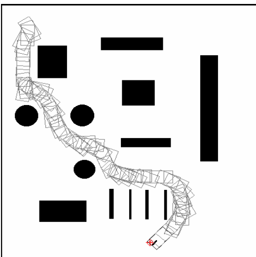
Fig. 9. Robot path in unknown environment
